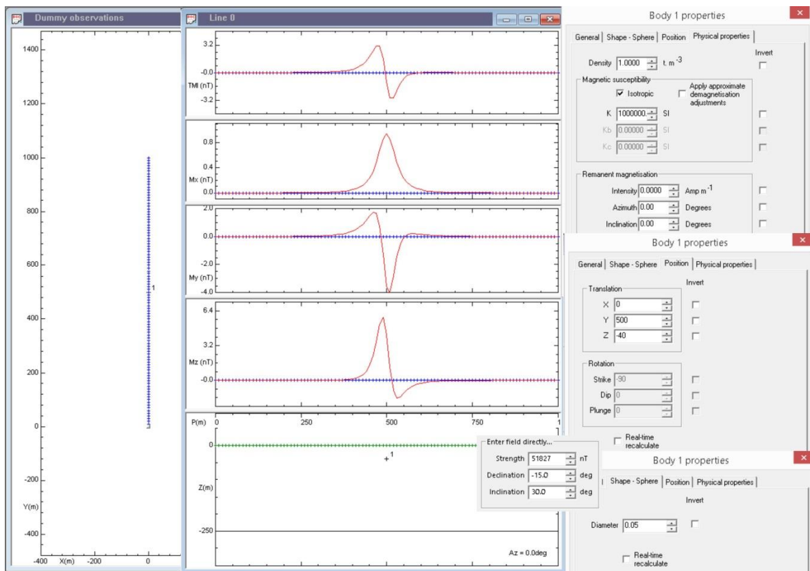
Figure 1.2 Potent v4.12.04 model's parameters and modeling results
