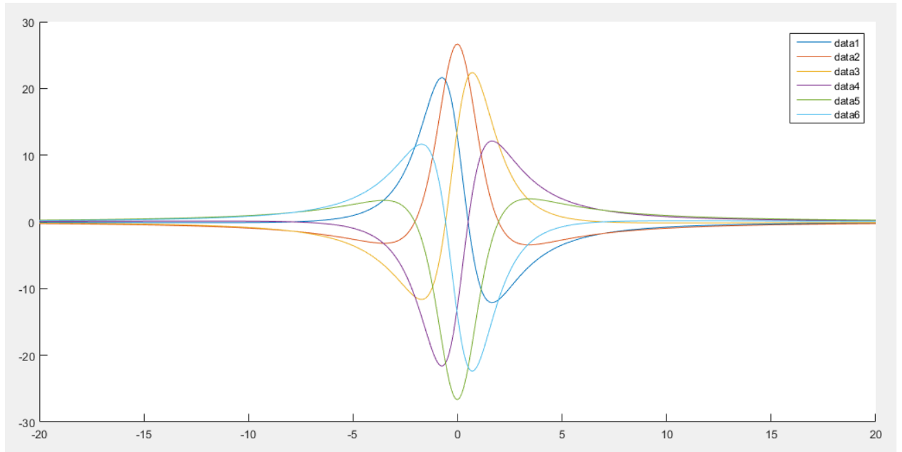
Figure 3.4 gMagyModCylinder using result for different magnetization direction (example 2)
