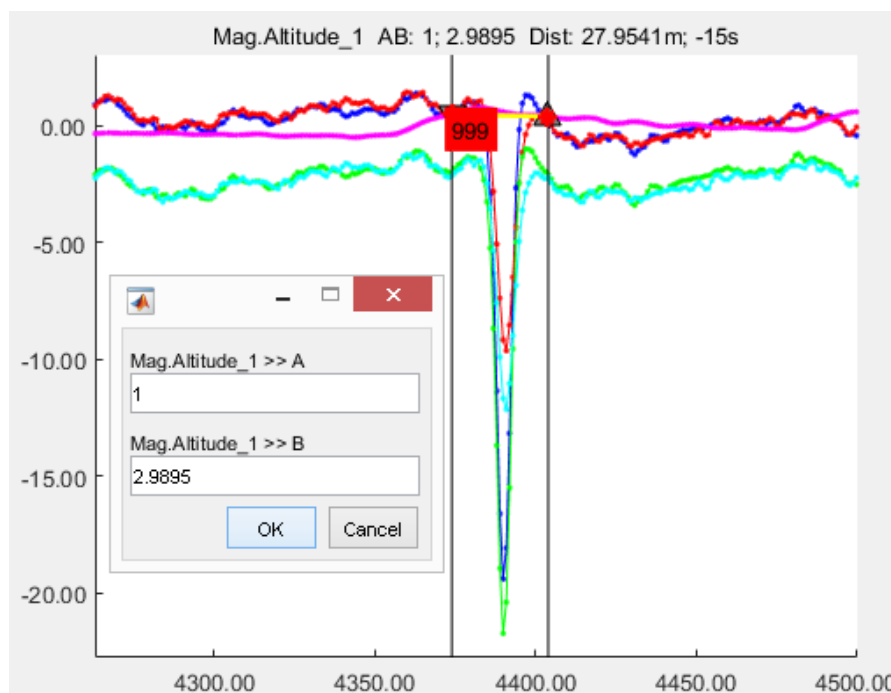
Figure 5.2 Zoomed GraphsWindow with target 999 picked and graph/scale selected window (key “s”)
