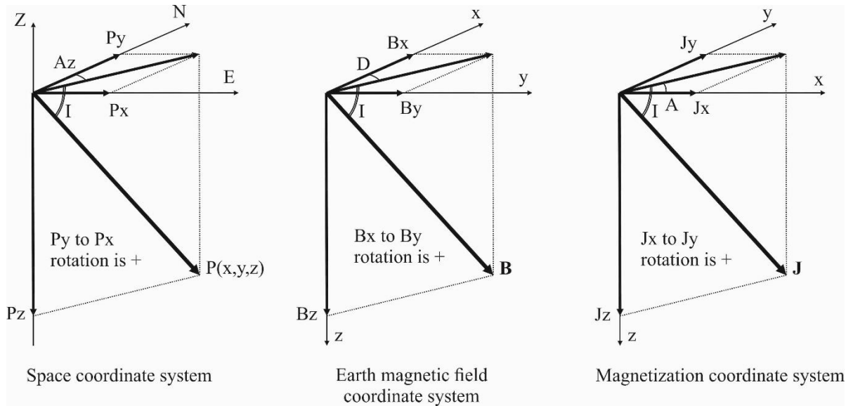
Figure 1.1 Magnetic parameters coordinate system
